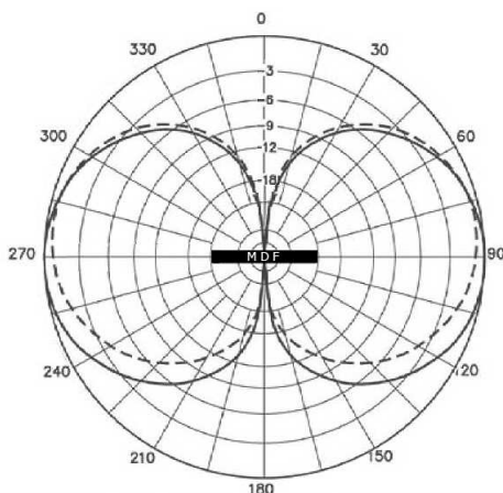
Typ. Antenna Pattern
